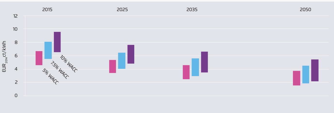
LCOE India (1400 - 1850 kWh/kWp p.a.); WACC between 5% and 10%
