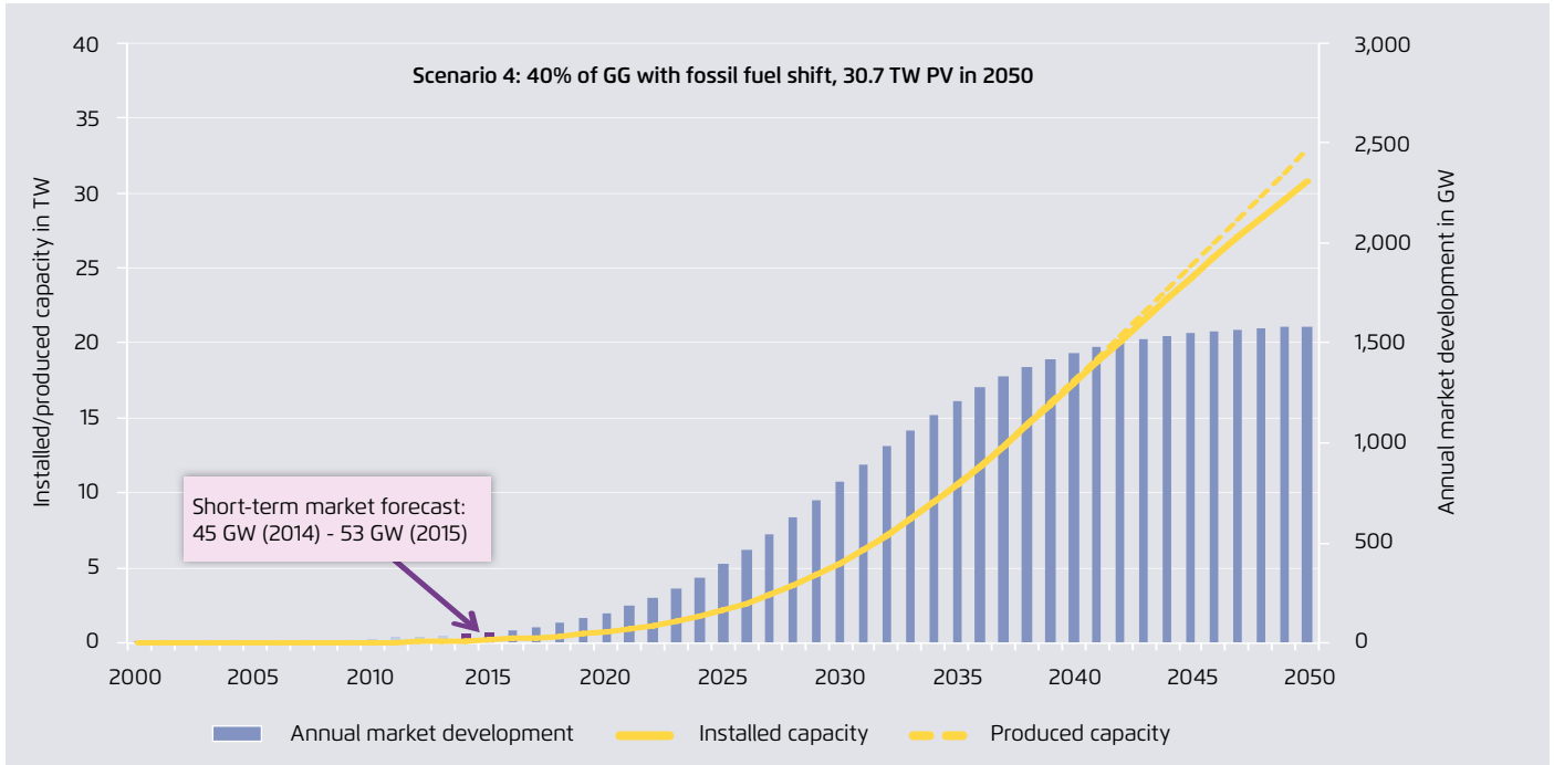
Installed and produced capacity, scenario 4
