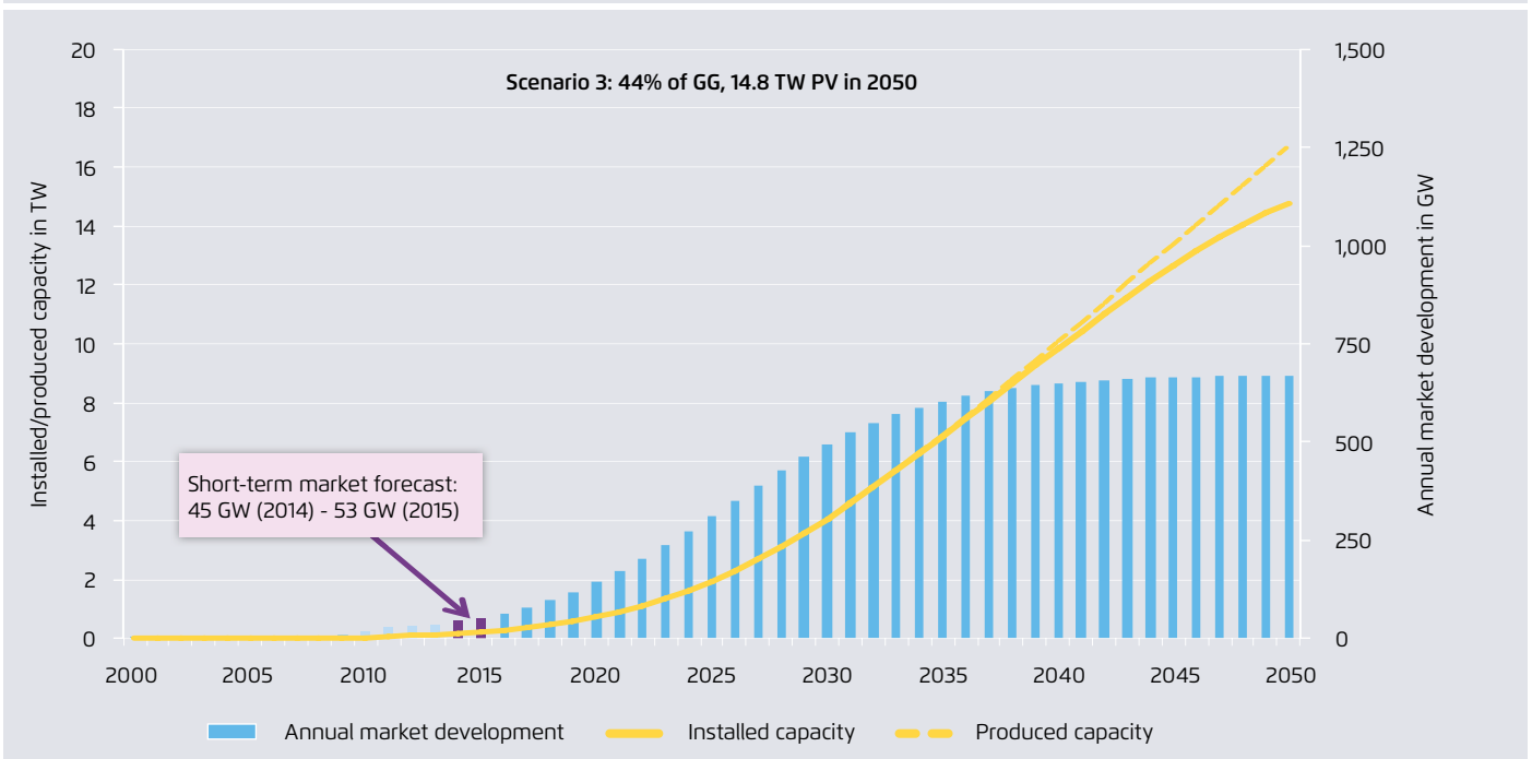
Installed and produced capacity, scenario 3
