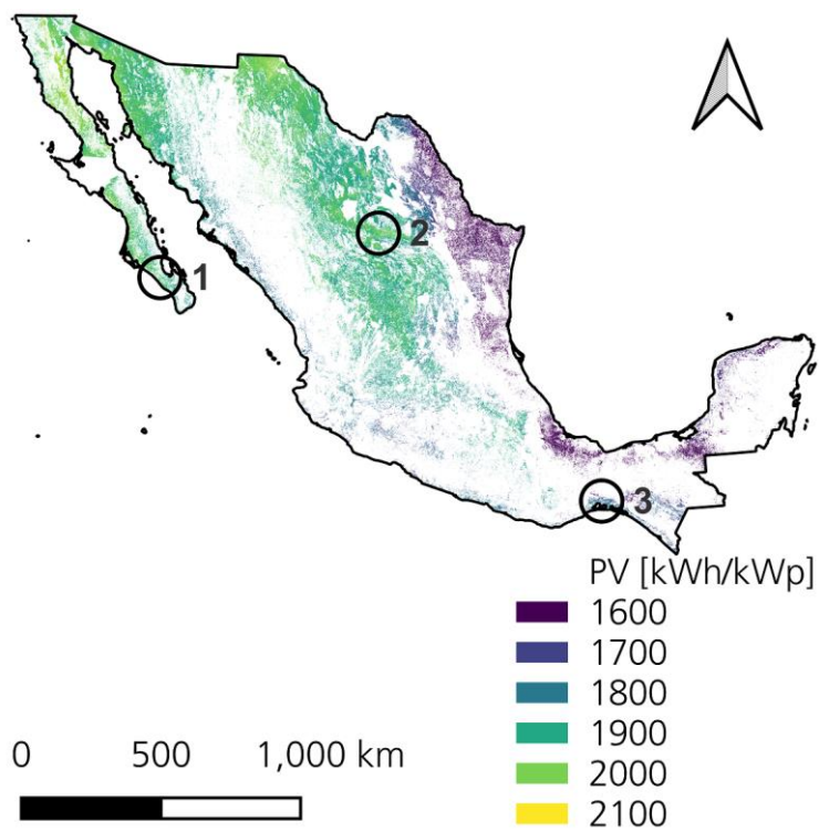
Figure 9-48: Selected regions and PV potential in Mexico.
