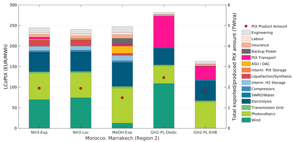
Figure 9-59: Cost breakdowns (left y-axis) and total PtX product amounts (right y-axis) for the Moroccan site “Marrakech” (Region 2) and the assessed PtX energy carriers and their local production (-Loc) or supply cost (-Exp) including transport to Germany. The costs shown here apply to the respective cost-optimal system layout. The respective energy demands of individual components (such as electrolysis or compressors) are included in the cost shares of wind and PV (and not in the cost share of the electrolysis or compressors). The reason is that the systems are almost exclusively supplied by the local dedicated wind and PV plants. Therefore, the energy demand of a specific component directly affects the installed capacities of wind and PV.
