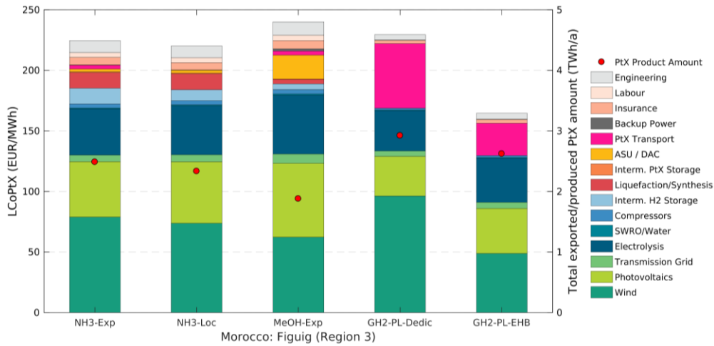
Figure 9-61: Cost breakdowns (left y-axis) and total PtX product amounts (right y-axis) for the Moroccan site “Figuiq” (Region 3) and the assessed PtX energy carriers and their local production (-Loc) or supply cost (-Exp) including transport to Germany. The costs shown here apply to the respective cost-optimal system layout. The respective energy demands of individual components (such as electrolysis or compressors) are included in the cost shares of wind and PV (and not in the cost share of the electrolysis or compressors). The reason is that the systems are almost exclusively supplied by the local dedicated wind and PV plants. Therefore, the energy demand of a specific component directly affects the installed capacities of wind and PV.
