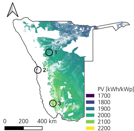
Figure 6-20: PV potential and selected regions in Namibia
