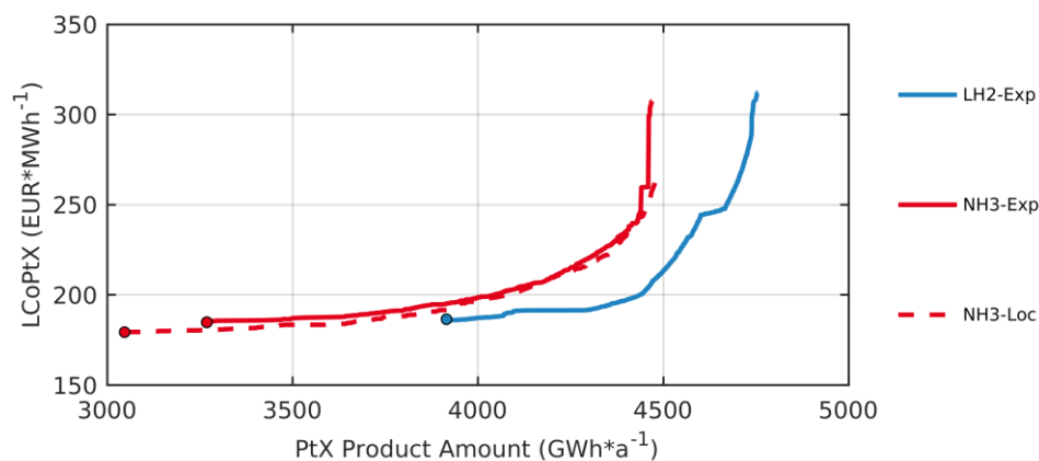
Figure 9-26: The Pareto fronts for the Brazilian site “Bahia North – Irece” (region 2) show the respective PtX supply costs (LcoPtX; incl. transport) identified in the optimization process as a function of the total PtX product amount. The PtX system designs and costs presented and discussed in this study always refer to the absolute cost optimum at the left end of the Pareto fronts. If a higher product amount (at a constant installed electrolysis capacity of 1 GW el ) is targeted at a site, this can be significantly increased in some cases with only a slight increase in PtX supply costs.
