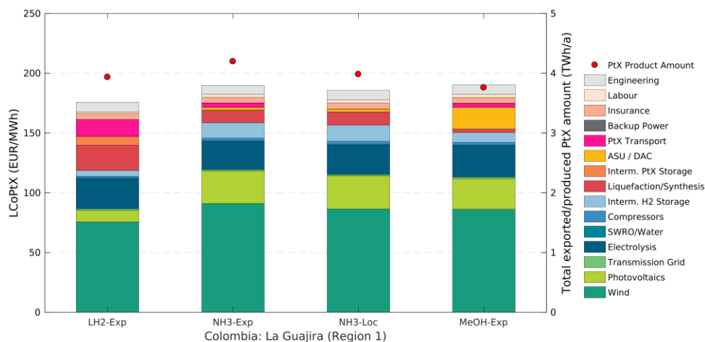
Figure 6-18: Cost breakdown and total PtX product amounts for the Colombian location Guajira/Uribea (Region 1) for four product scenarios exported liquid hydrogen (LH2-Exp), exported ammonia and methanol (NH3-Exp, MeOH-Exp) and the local distribution of ammonia (NH3-Loc). The costs shown here apply to the respective cost-optimal system layout.
