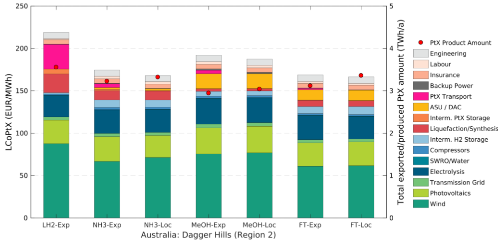
Figure 6-24: Cost breakdown and total PtX product amounts for the Western Australian region Dagger Hills (Region 2) for the seven product scenarios - exported liquid hydrogen (LH 2 -Exp), as well as the exported and local scenarios for ammonia, methanol and Fischer-Tropsch products (NH 3 -Exp, MeOH-Exp, FT-Exp and NH 3 -Loc, MeOH-Loc, FT-Loc, respectively). The costs shown here apply to the respective cost-optimal system layout.
