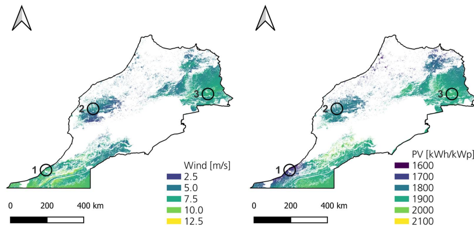
Figure 6-26: Wind potential and selected regions in Morocco
