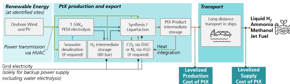
Figure 3-1: System layout for the liquid PtX products liquid hydrogen, ammonia, methanol and jet fuel. Renewable electricity is generated via onshore wind and photovoltaics at sites identified through GIS analyses. Subsequently the electricity is transported to the site of PtX production and export, usually near an existing port with sufficient draft and capacity. Subsequently, the products are either considered for the local market or transported by ship to the target port in Brunsbüttel, Germany.
