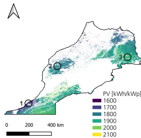
Figure 6-27: PV potential and selected regions in Morocco
