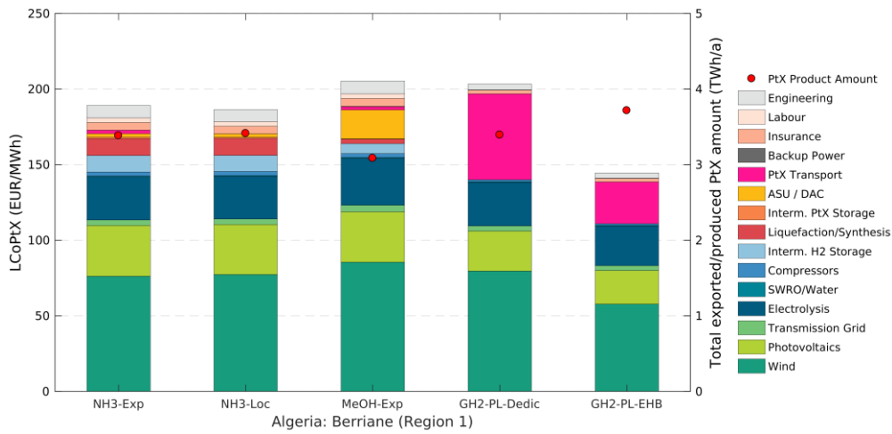
Figure 9-3: Cost breakdowns (left y-axis) and total PtX product amounts (right y-axis) for the Algerian site “Berriane” (Region 1) and the assessed PtX energy carriers and their local production (-Loc) or supply cost (-Exp) including transport to Germany. The costs shown here apply to the respective cost-optimal system layout. The respective energy demands of individual components (such as electrolysis or compressors) are included in the cost shares of wind and PV (and not in the cost share of the electrolysis or compressors). The reason is that the systems are almost exclusively supplied by the local dedicated wind and PV plants. Therefore, the energy demand of a specific component directly affects the installed capacities of wind and PV.
