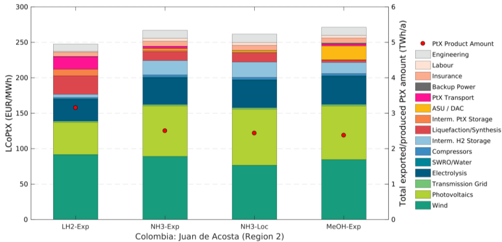
Figure 9-33: Cost breakdowns (left y-axis) and total PtX product amounts (right y-axis) for the Colombian site “Juan de Acosta” (Region 2) and the assessed PtX energy carriers and their local production (-Loc) or supply cost (-Exp) including transport to Germany. The costs shown here apply to the respective cost-optimal system layout. The respective energy demands of individual components (such as electrolysis or compressors) are included in the cost shares of wind and PV (and not in the cost share of the electrolysis or compressors). The reason is that the systems are almost exclusively supplied by the local dedicated wind and PV plants. Therefore, the energy demand of a specific component directly affects the installed capacities of wind and PV.
