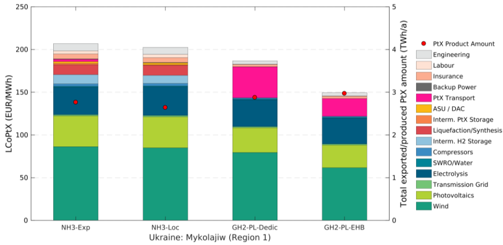
Figure 9-97: Cost breakdowns (left y-axis) and total PtX product amounts (right y-axis) for the Ukrainian site “Mykolaiv” (Region 1) and the assessed PtX energy carriers and their local production (-Loc) or supply cost (-Exp) including transport to Germany. The costs shown here apply to the respective cost-optimal system layout. The respective energy demands of individual components (such as electrolysis or compressors) are included in the cost shares of wind and PV (and not in the cost share of the electrolysis or compressors). The reason is that the systems are almost exclusively supplied by the local dedicated wind and PV plants. Therefore, the energy demand of a specific component directly affects the installed capacities of wind and PV.
