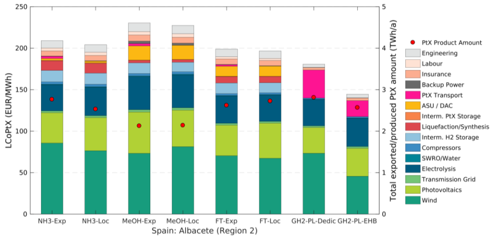
Figure 9-83: Cost breakdowns (left y-axis) and total PtX product amounts (right y-axis) for the Spanish site “Albacete” (Region 2) and the assessed PtX energy carriers and their local production (-Loc) or supply cost (-Exp) including transport to Germany. The costs shown here apply to the respective cost-optimal system layout. The respective energy demands of individual components (such as electrolysis or compressors) are included in the cost shares of wind and PV (and not in the cost share of the electrolysis or compressors). The reason is that the systems are almost exclusively supplied by the local dedicated wind and PV plants. Therefore, the energy demand of a specific component directly affects the installed capacities of wind and PV.
