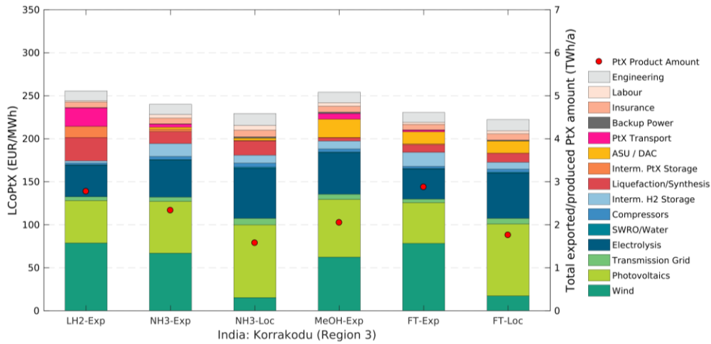
Figure 9-43: Cost breakdowns (left y-axis) and total PtX product amounts (right y-axis) for the Indian site “Korarakodu” (Region 3) and the assessed PtX energy carriers and their local production (-Loc) or supply cost (-Exp) including transport to Germany. The costs shown here apply to the respective cost-optimal system layout. The respective energy demands of individual components (such as electrolysis or compressors) are included in the cost shares of wind and PV (and not in the cost share of the electrolysis or compressors). The reason is that the systems are almost exclusively supplied by the local dedicated wind and PV plants. Therefore, the energy demand of a specific component directly affects the installed capacities of wind and PV.
