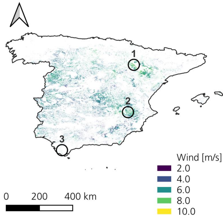
Figure 9-79: Selected regions and wind potential in Spain.
