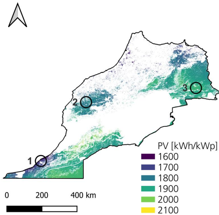
Figure 9-56: Selected regions and PV potential in Morocco.
