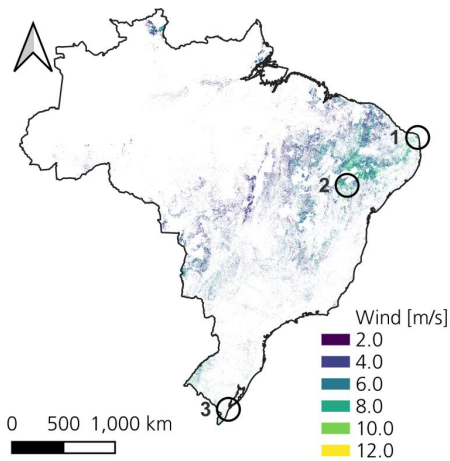
Figure 6-13: Wind potential and selected regions in Brazil
