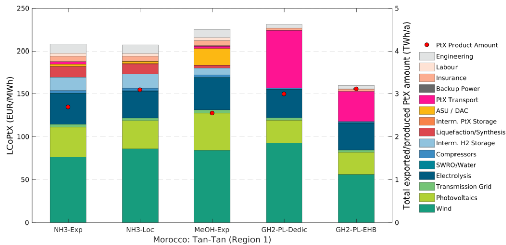
Figure 6-28: Cost breakdown and total product amounts for the Moroccan location Tan-Tan (Region 1) for five product scenarios exported ammonia and methanol (NH 3 -Exp, MeOH-Exp), local distribution of ammonia (NH 3 -Loc), and gaseous hydrogen either transported in dedicated hydrogen pipelines (GH 2 -PL-Dedic) or transported in an expanded European Hydrogen Backbone (GH 2 -PL-EHB). The costs shown here apply to the respective cost-optimal system layout.
