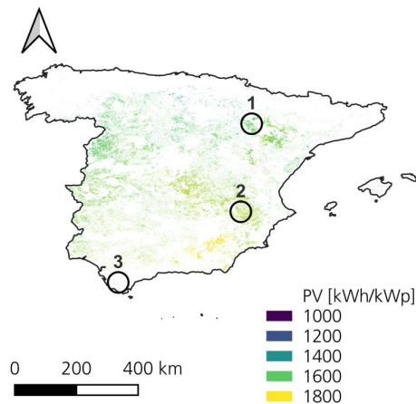
Figure 6-30: PV potential and selected regions in Spain
